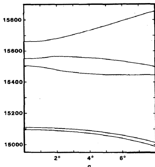
Fig. 7. Calculated ( {}^2E_g , {}^2T_{1g} ) transition energies for a trigonally distorted \text{CrN}_5\text{Cl} chromophore as a function of the cartesian bite angle. e_{\sigma\text{N}} = 7000 , e_{\sigma\text{Cl}} = 6400 , e_{\pi\text{Cl}} = 900 .
