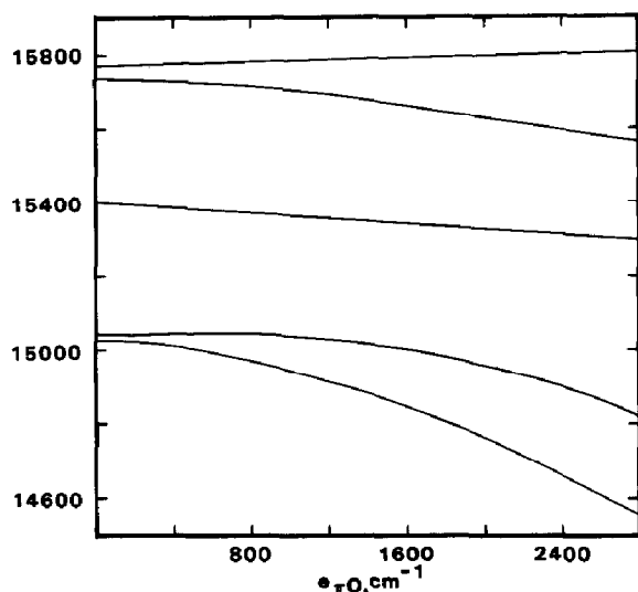
Fig. 9. Calculated ( {}^2E_g , {}^2T_{1g} ) transition energies for fac -[Cr(gly) 3 ] as a function of e_{\pi O} (anisotropic). e_{\sigma N} = 7000 , e_{\sigma O} = \frac{1}{3}(19,500 - 2e_{\pi O}) .
