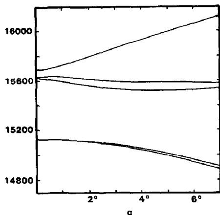
Fig. 6. Calculated ( {}^2E_g , {}^2T_{1g} ) transition energies for a [\text{Cr}(\overline{\text{N-N-N}})_2]^{3+} complex as a function of the trigonal cartesian bite angle. e_{\sigma\text{N}} = 7000 , \beta = 0 .
