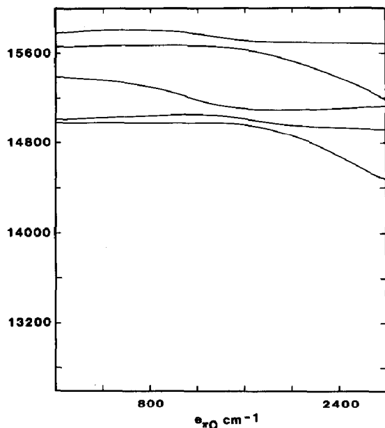
Fig. 1. Calculated ( {}^2E_g, {}^2T_{1g} ) transition energies for \text{K}[\text{Cr}(\text{IDA})_2] as a function of an isotropic e_{\pi O} , e_{\sigma N} = 7000 , e_{\sigma O} = \frac{1}{3}(19,500 - 4e_{\pi O}) , B = 650 , C = 2650 , \zeta = 250 , \alpha = 0 . The last four values are used in all subsequent energy plots.
